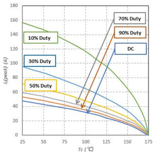
Fig.7-Current Derating
