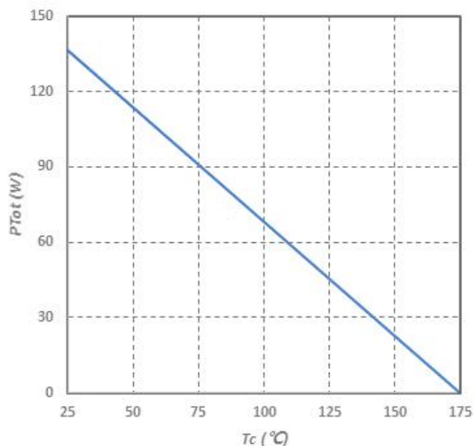
Fig.6-Power Derating
